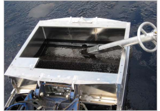
The Doro skimmer can be used with or without Sala Roll Pump. The Doro skimmer holds approx. 20 litres.
