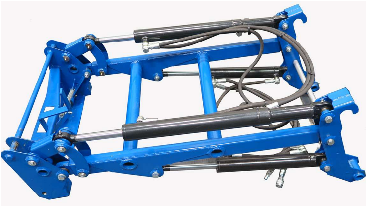
Lifting arm with parallel movement. Semi-automatic quick bracket X4 for fast tool replacement.
